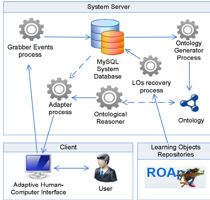
Fig. 1. HCI Interface model proposed
