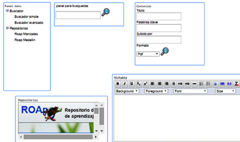
Fig. 3. GUI Deployment
