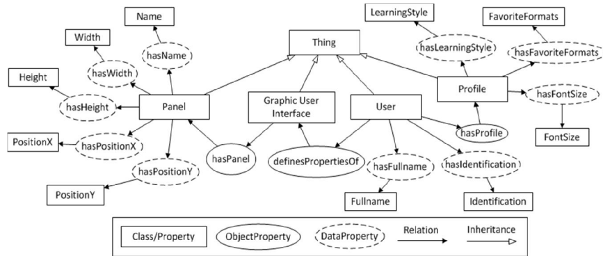
Fig. 2. GUI & User-profile ontological structure
